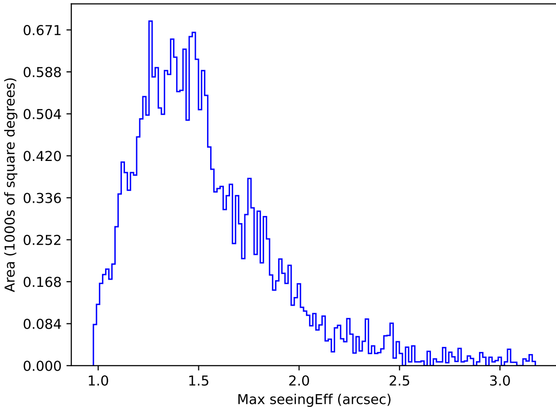
too_ignore_5_1v3.4_10yrs Yr 1 g band: Max seeingEff
