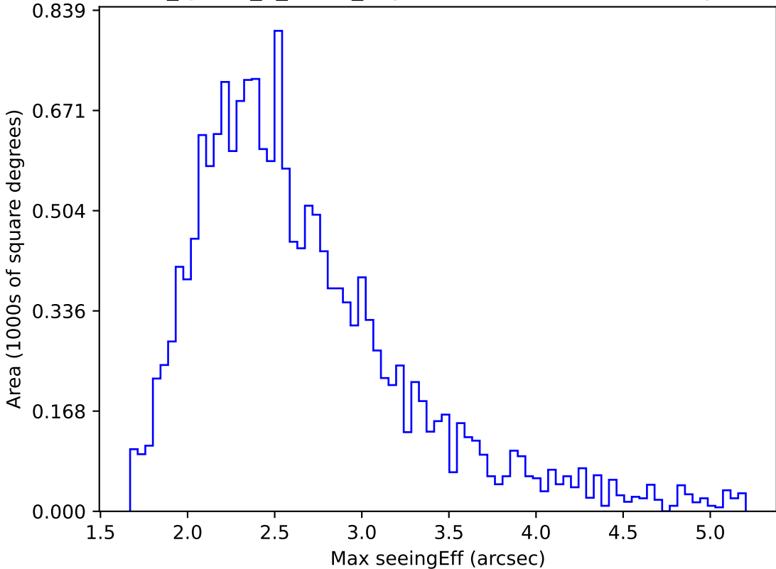
too_ignore_5_1v3.4_10yrs WFD z band: Max seeingEff
