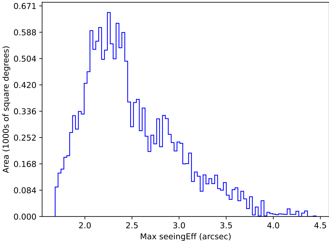
too_ignore_5_1v3.4_10yrs WFD u band: Max seeingEff
