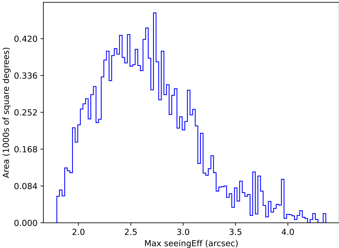
too_ignore_5_1v3.4_10yrs WFD r band: Max seeingEff
