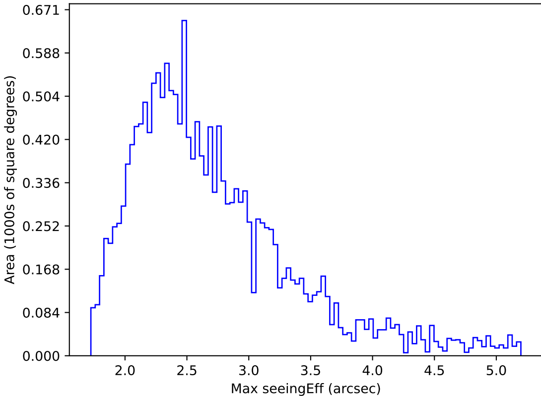
too_ignore_5_1v3.4_10yrs WFD i band: Max seeingEff
