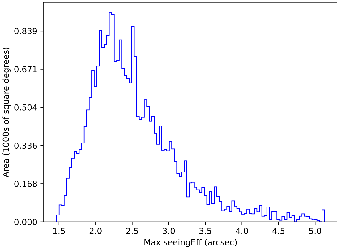
too_ignore_5_1v3.4_10yrs All sky z band: Max seeingEff
