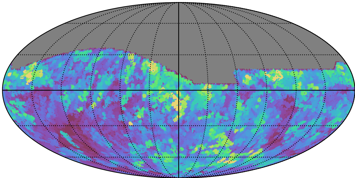
too_ignore_5_1v3.4_10yrs All sky r band: Max seeingEff
