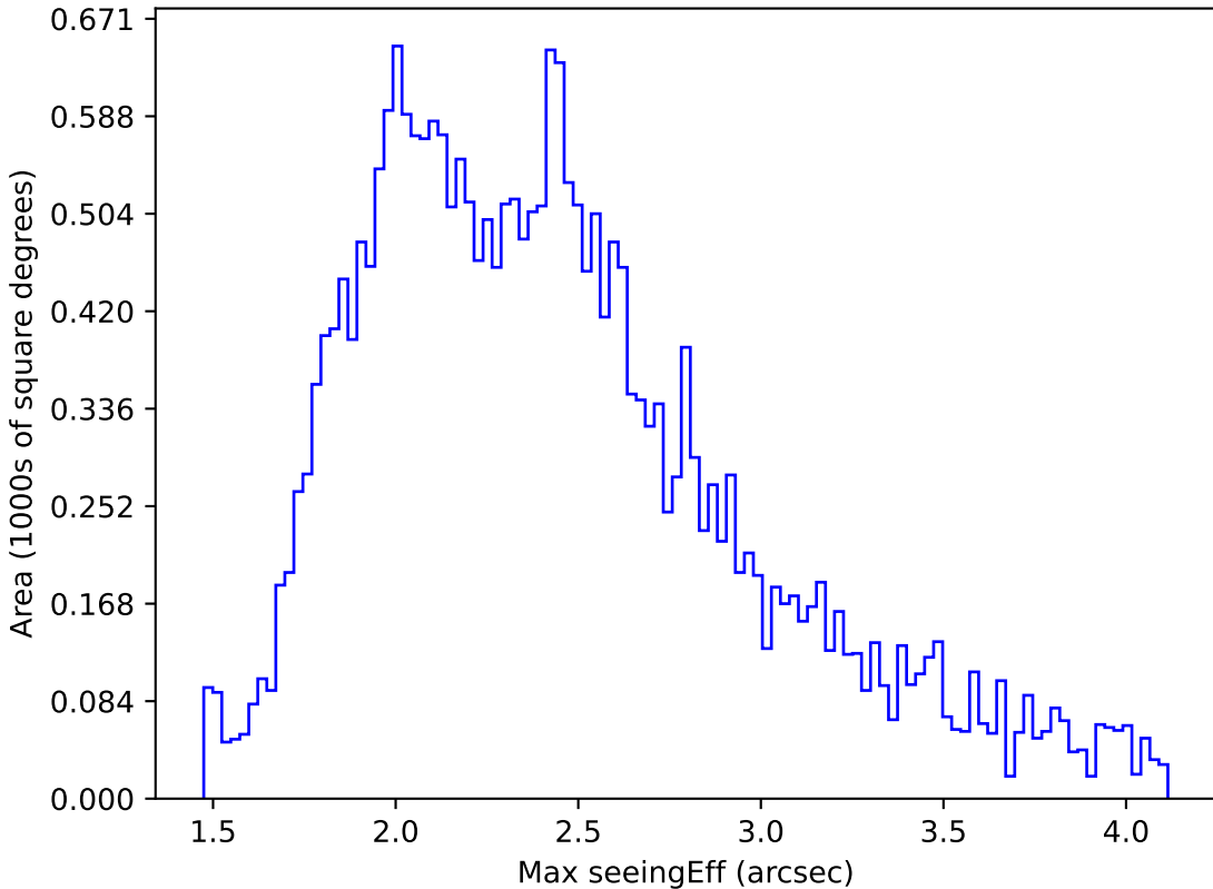
too_ignore_5_1v3.4_10yrs All sky g band: Max seeingEff
