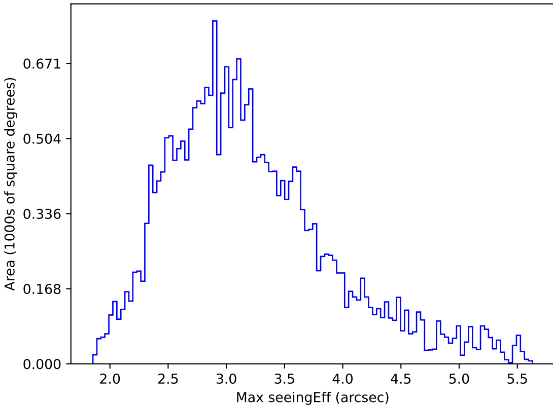
too_ignore_5_1v3.4_10yrs All sky all bands: Max seeingEff
