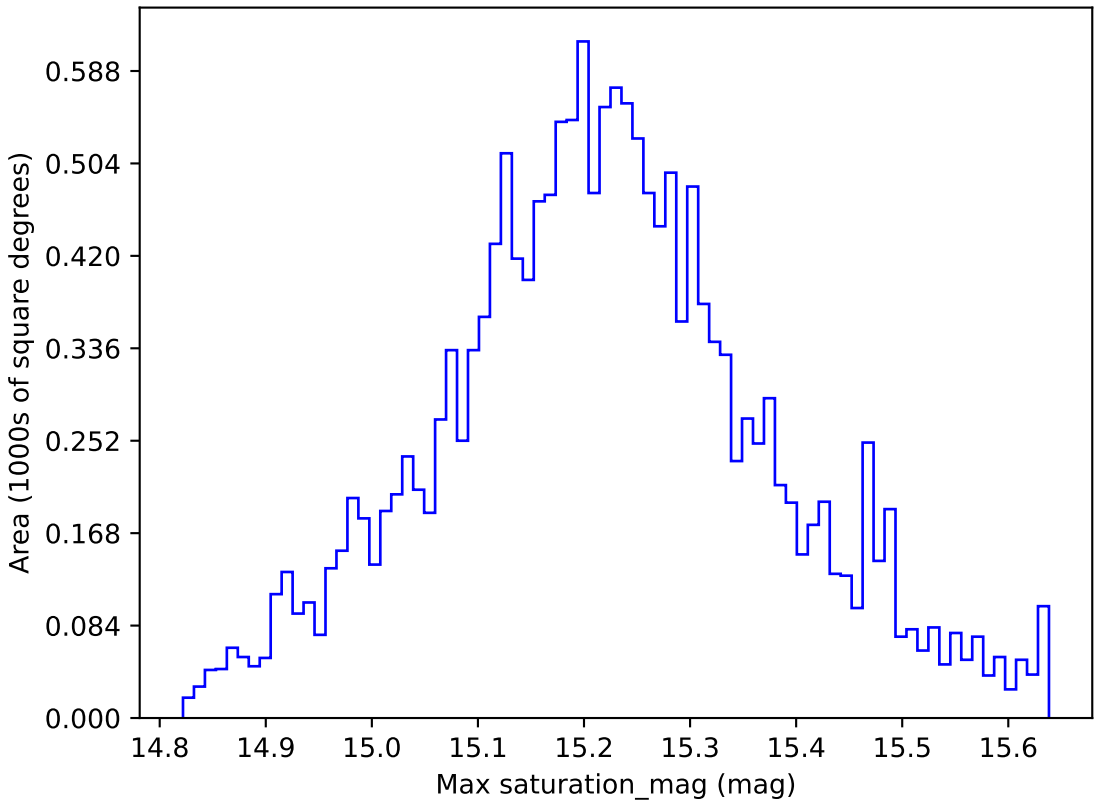
too_ignore_5_1v3.4_10yrs WFD z band: Max saturation_mag
