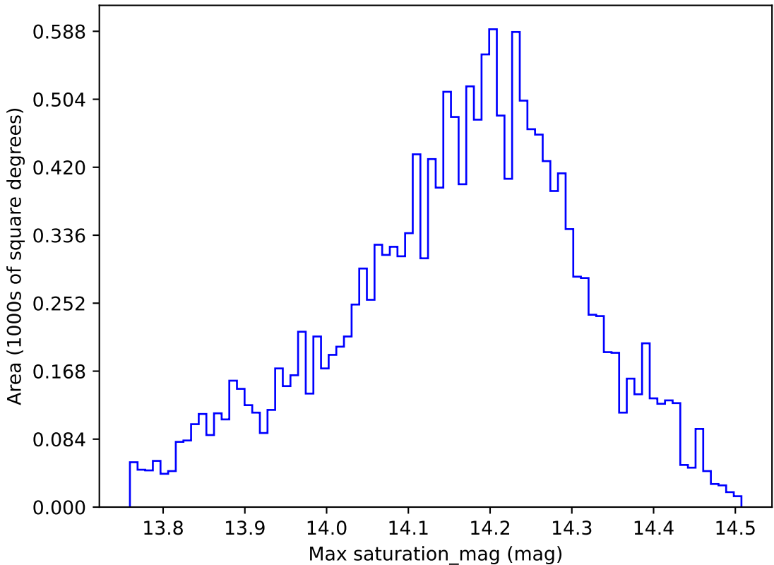
too_ignore_5_1v3.4_10yrs WFD y band: Max saturation_mag
