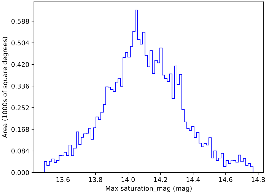
too_ignore_5_1v3.4_10yrs WFD u band: Max saturation_mag
