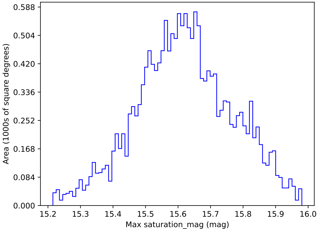
too_ignore_5_1v3.4_10yrs WFD i band: Max saturation_mag
