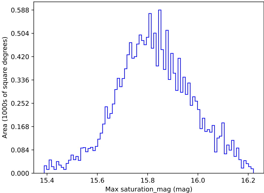
too_ignore_5_1v3.4_10yrs WFD all bands: Max saturation_mag
