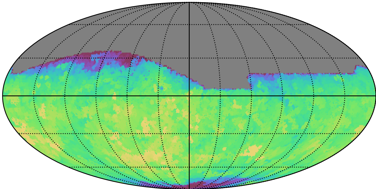
too_ignore_5_1v3.4_10yrs All sky r band: Max saturation_mag
