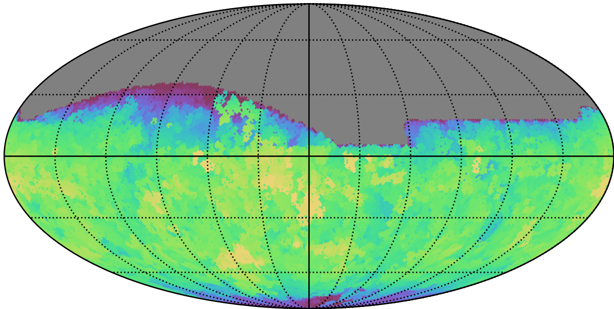
too_ignore_5_1v3.4_10yrs All sky g band: Max saturation_mag
