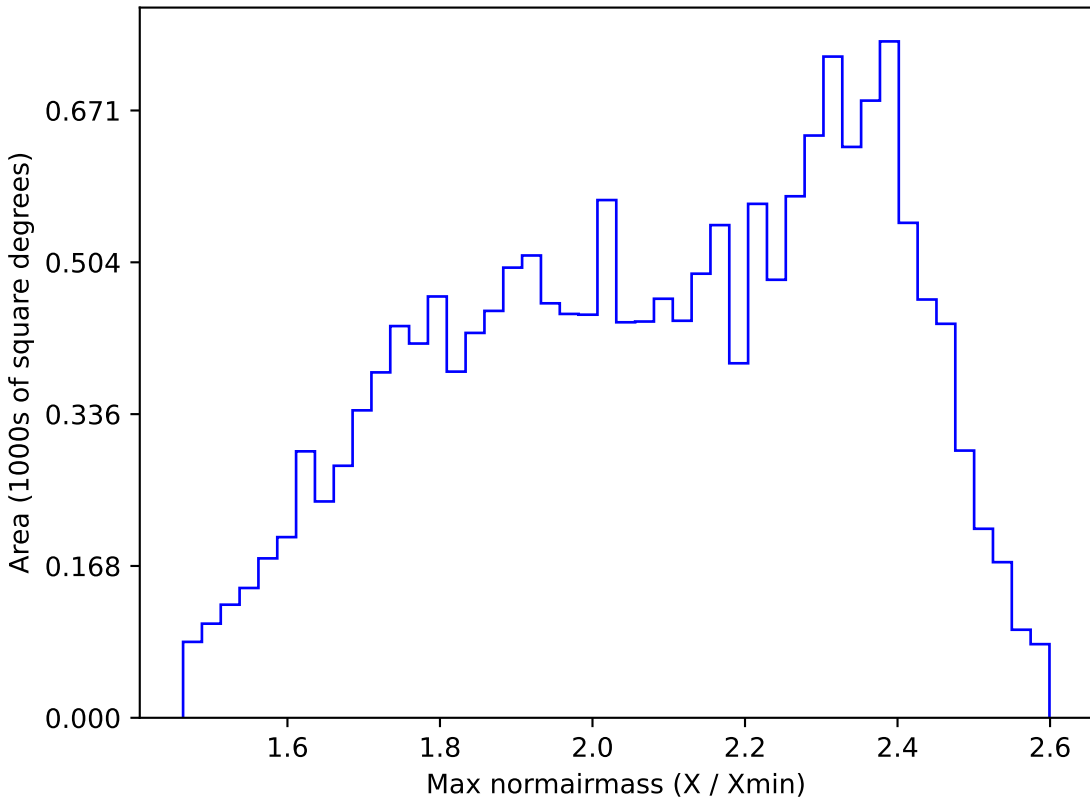
too_ignore_5_1v3.4_10yrs WFD r band: Max normairmass
