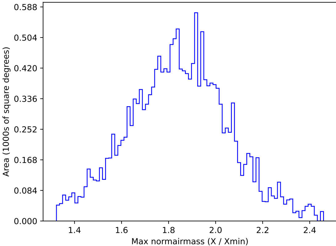
too_ignore_5_1v3.4_10yrs WFD g band: Max normairmass
