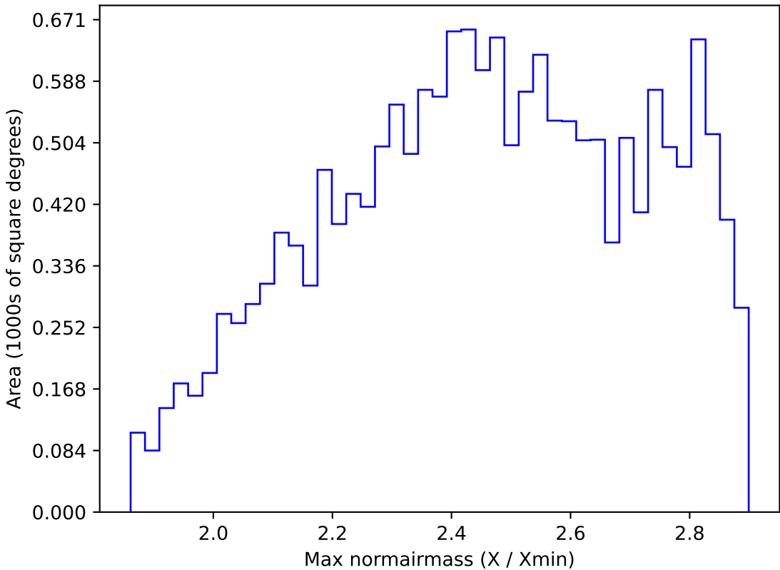
too_ignore_5_1v3.4_10yrs WFD all bands: Max normairmass
