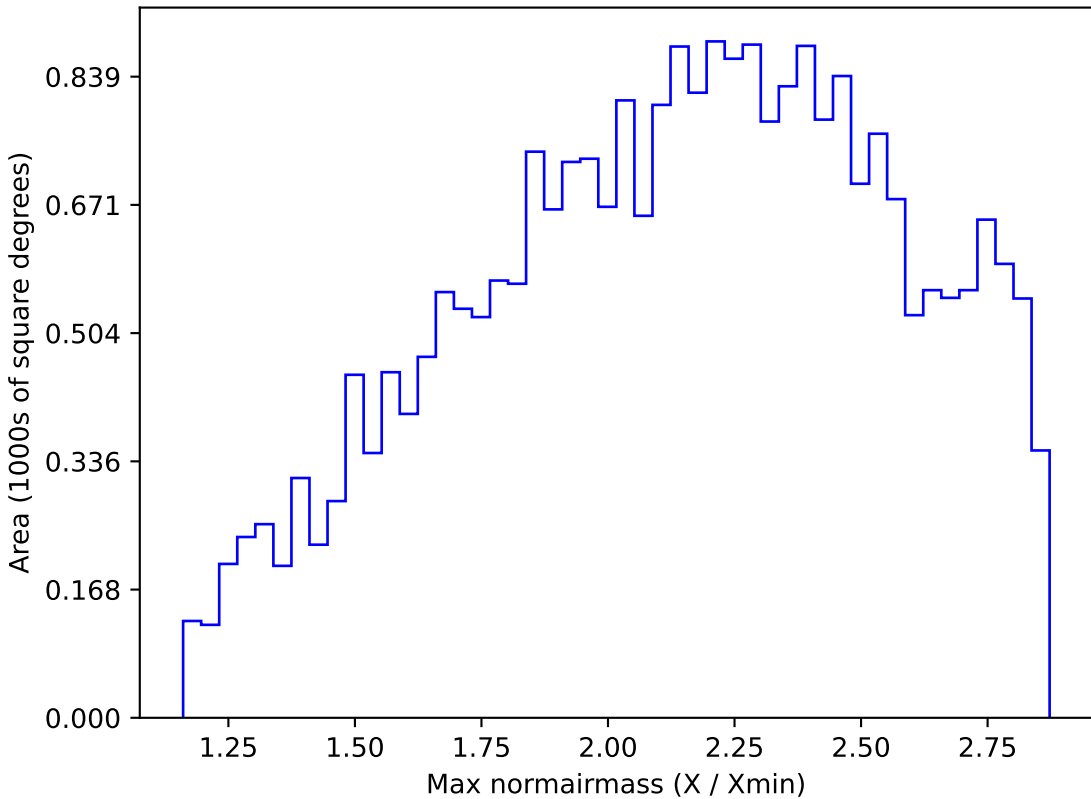
too_ignore_5_1v3.4_10yrs All sky z band: Max normairmass
