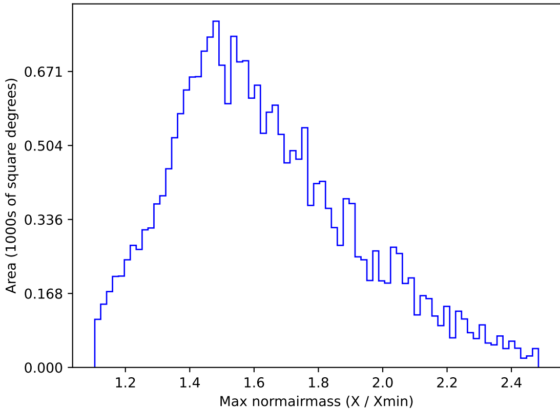
too_ignore_5_1v3.4_10yrs All sky u band: Max normairmass
