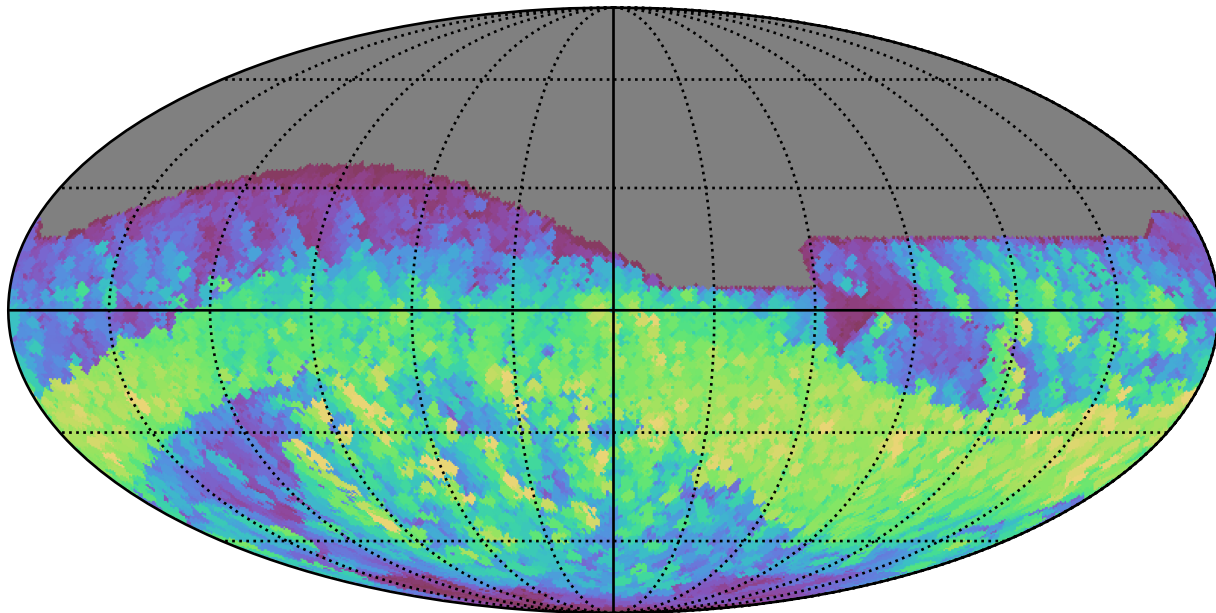
too_ignore_5_1v3.4_10yrs All sky r band: Max normairmass
