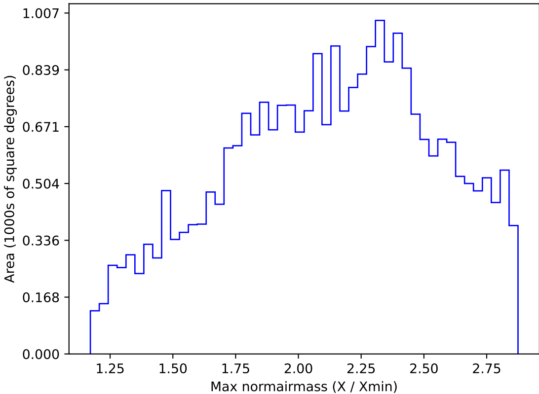
too_ignore_5_1v3.4_10yrs All sky i band: Max normairmass
