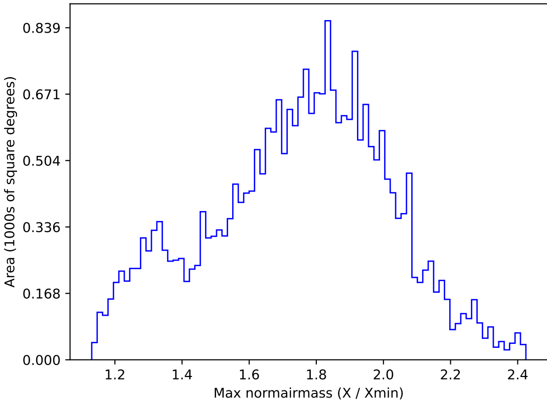
too_ignore_5_1v3.4_10yrs All sky g band: Max normairmass
