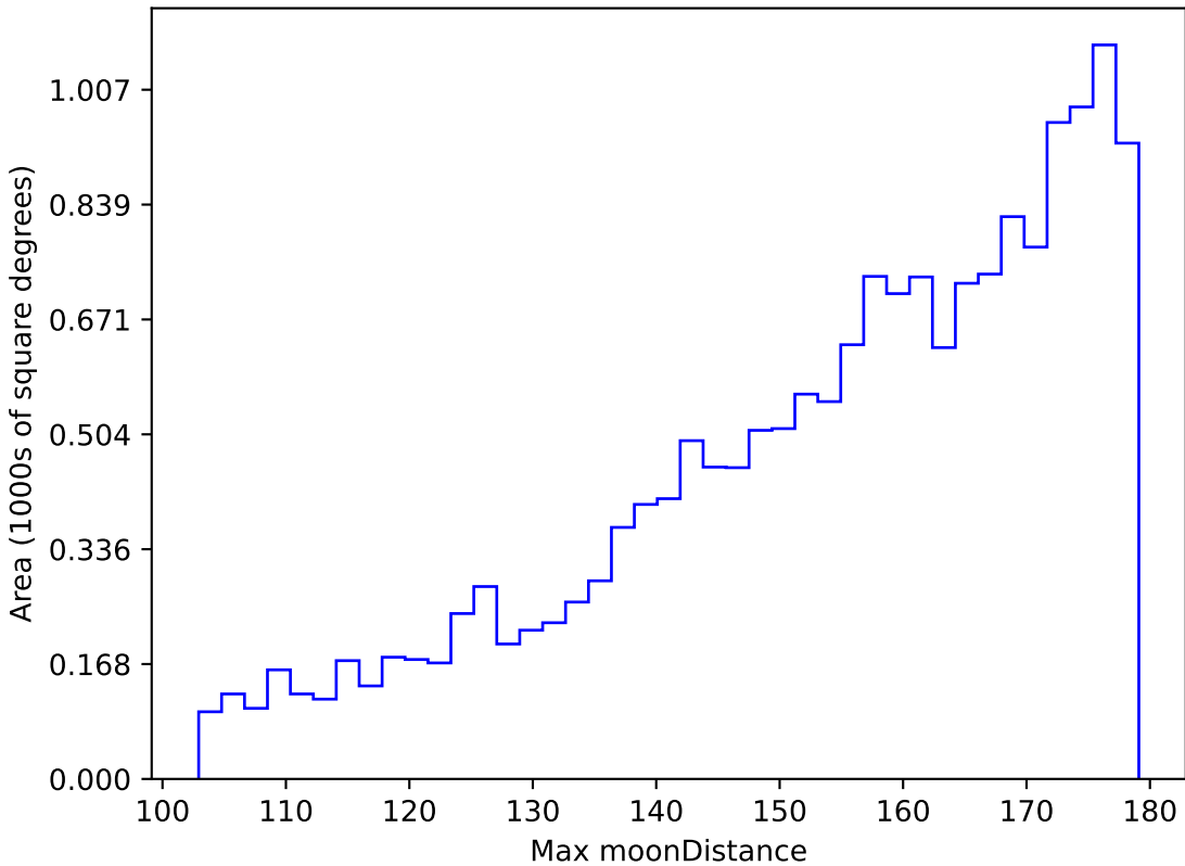
too_ignore_5_1v3.4_10yrs WFD z band: Max moonDistance
