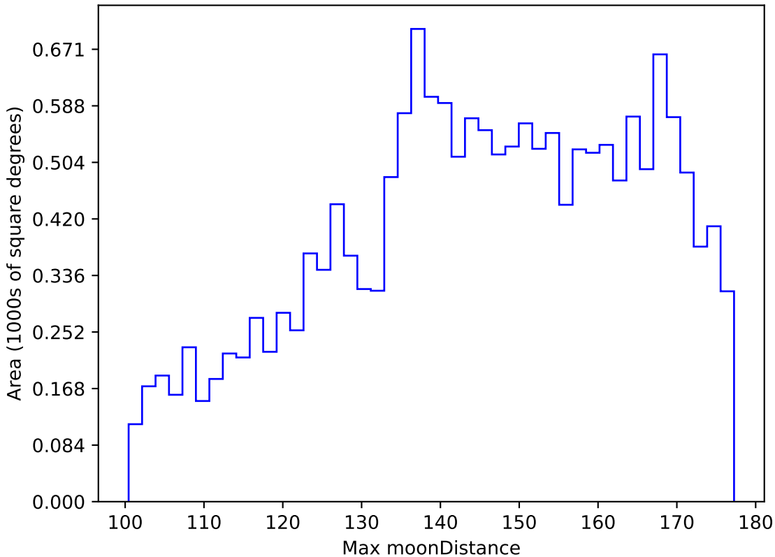
too_ignore_5_1v3.4_10yrs WFD y band: Max moonDistance
