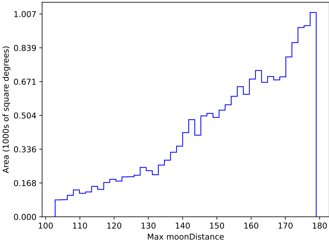
too_ignore_5_1v3.4_10yrs WFD u band: Max moonDistance
