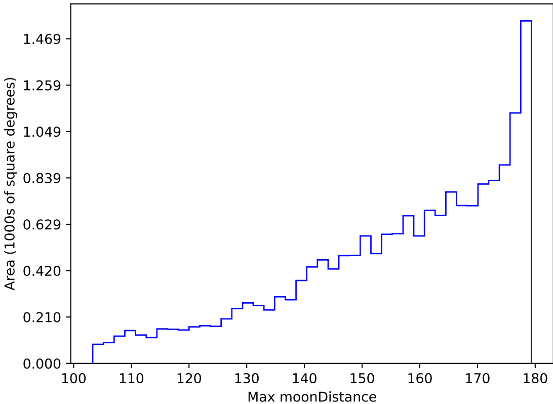
too_ignore_5_1v3.4_10yrs WFD r band: Max moonDistance
