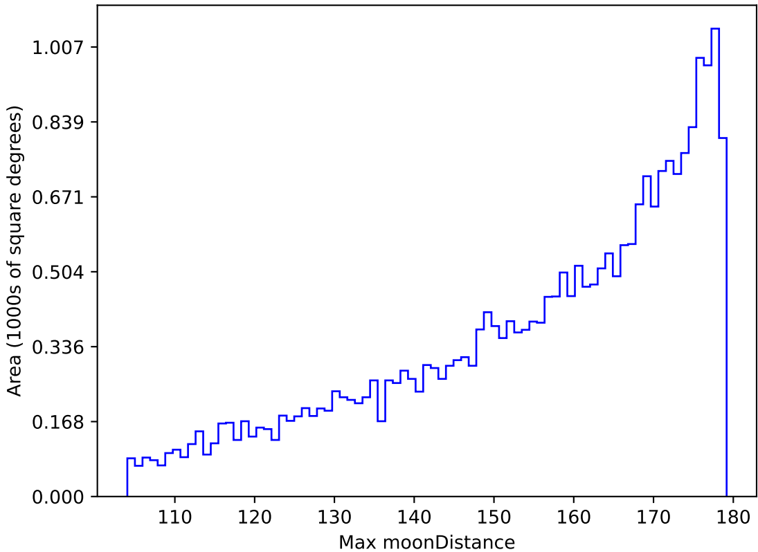
too_ignore_5_1v3.4_10yrs All sky i band: Max moonDistance
