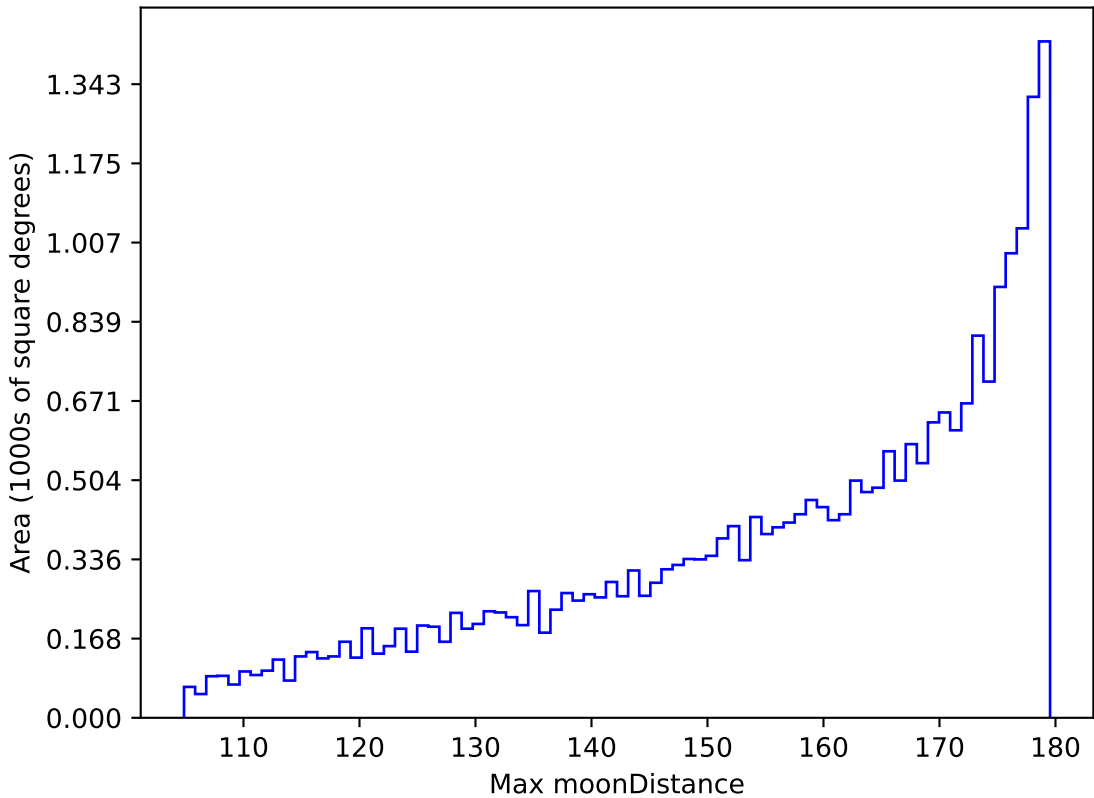
too_ignore_5_1v3.4_10yrs All sky all bands: Max moonDistance
