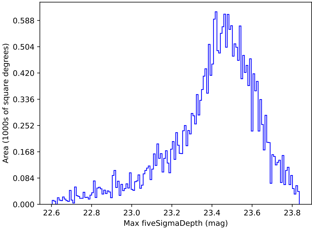
too_ignore_5_1v3.4_10yrs Yr 1 z band: Max fiveSigmaDepth
