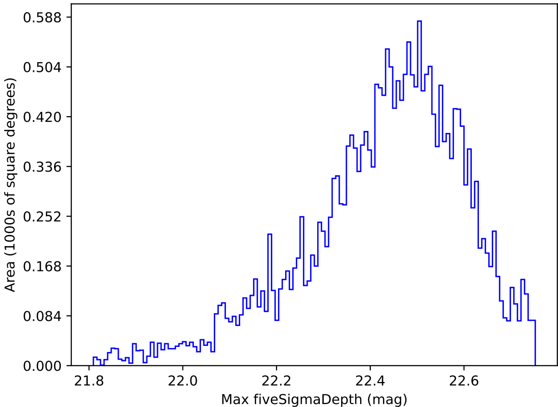
too_ignore_5_1v3.4_10yrs Yr 1 y band: Max fiveSigmaDepth
