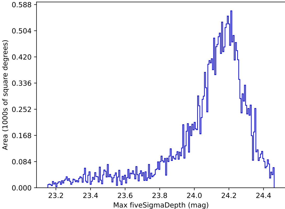
too_ignore_5_1v3.4_10yrs Yr 1 i band: Max fiveSigmaDepth
