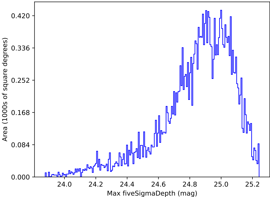
too_ignore_5_1v3.4_10yrs Yr 1 all bands: Max fiveSigmaDepth
