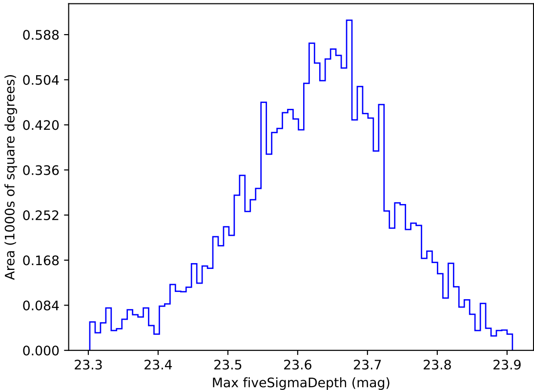
too_ignore_5_1v3.4_10yrs WFD z band: Max fiveSigmaDepth
