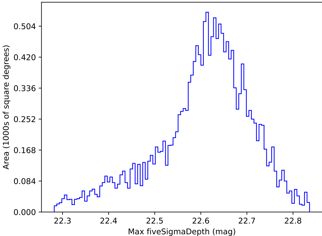
too_ignore_5_1v3.4_10yrs WFD y band: Max fiveSigmaDepth
