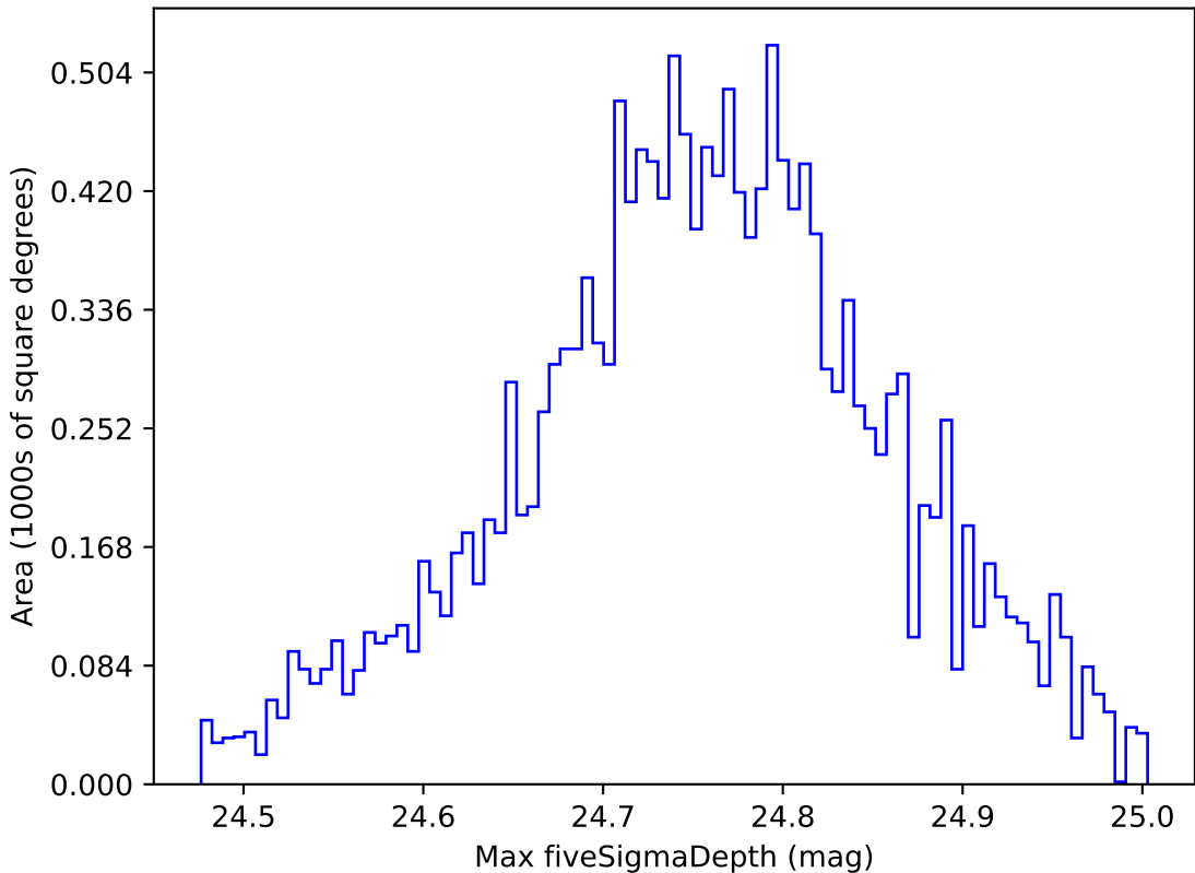
too_ignore_5_1v3.4_10yrs WFD r band: Max fiveSigmaDepth
