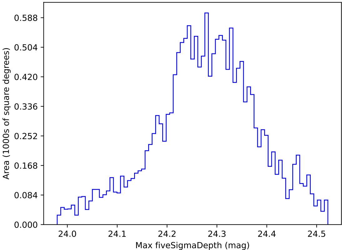
too_ignore_5_1v3.4_10yrs WFD i band: Max fiveSigmaDepth
