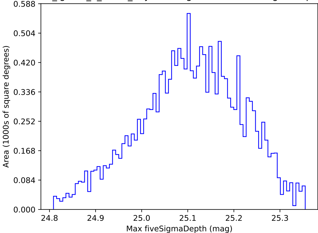
too_ignore_5_1v3.4_10yrs WFD g band: Max fiveSigmaDepth
