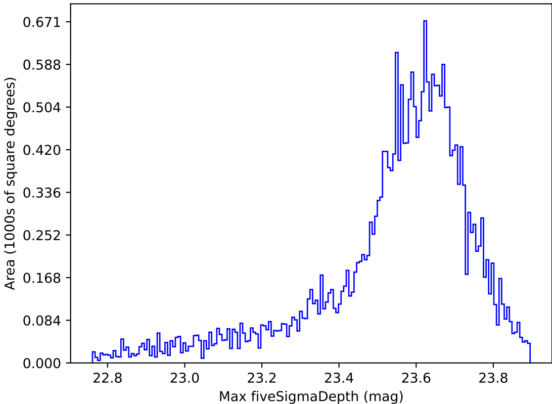
too_ignore_5_1v3.4_10yrs All sky z band: Max fiveSigmaDepth
