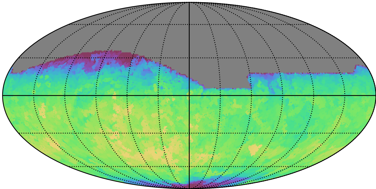
too_ignore_5_1v3.4_10yrs All sky r band: Max fiveSigmaDepth
