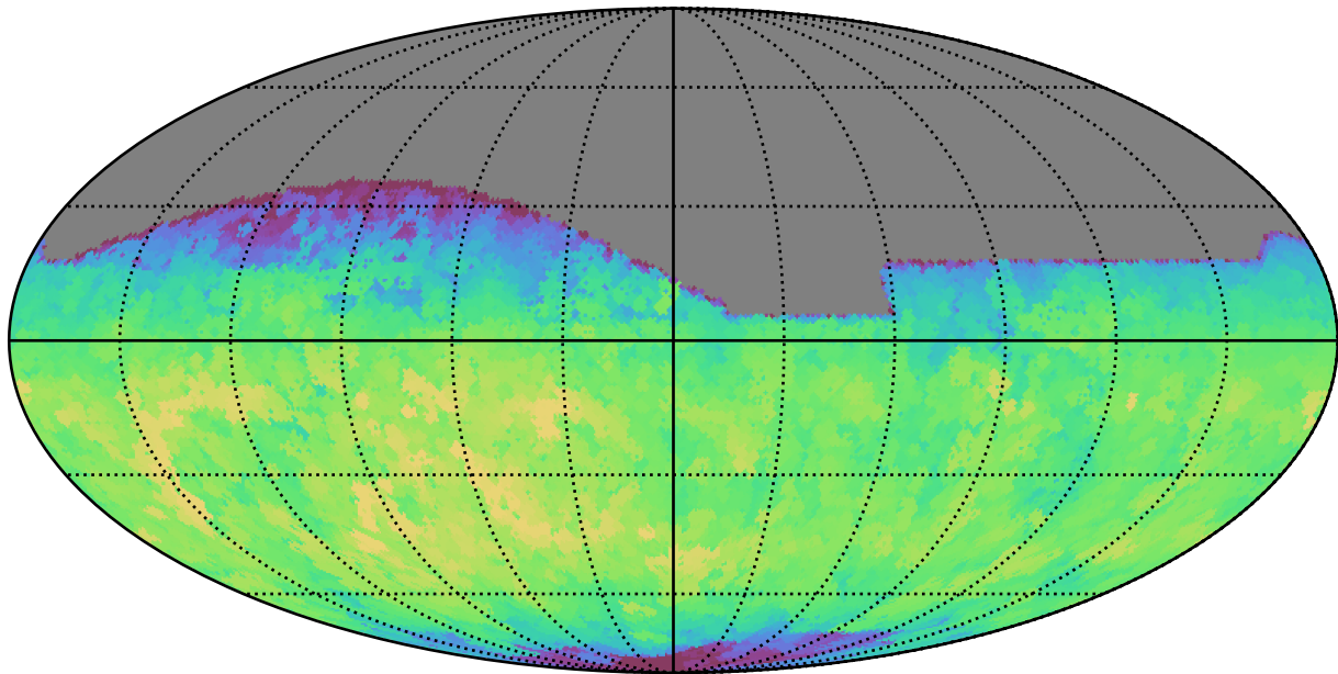
too_ignore_5_1v3.4_10yrs All sky i band: Max fiveSigmaDepth
