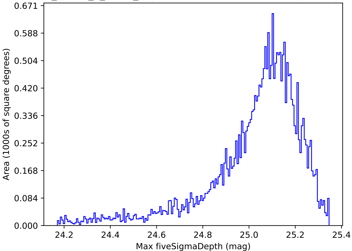
too_ignore_5_1v3.4_10yrs All sky g band: Max fiveSigmaDepth
