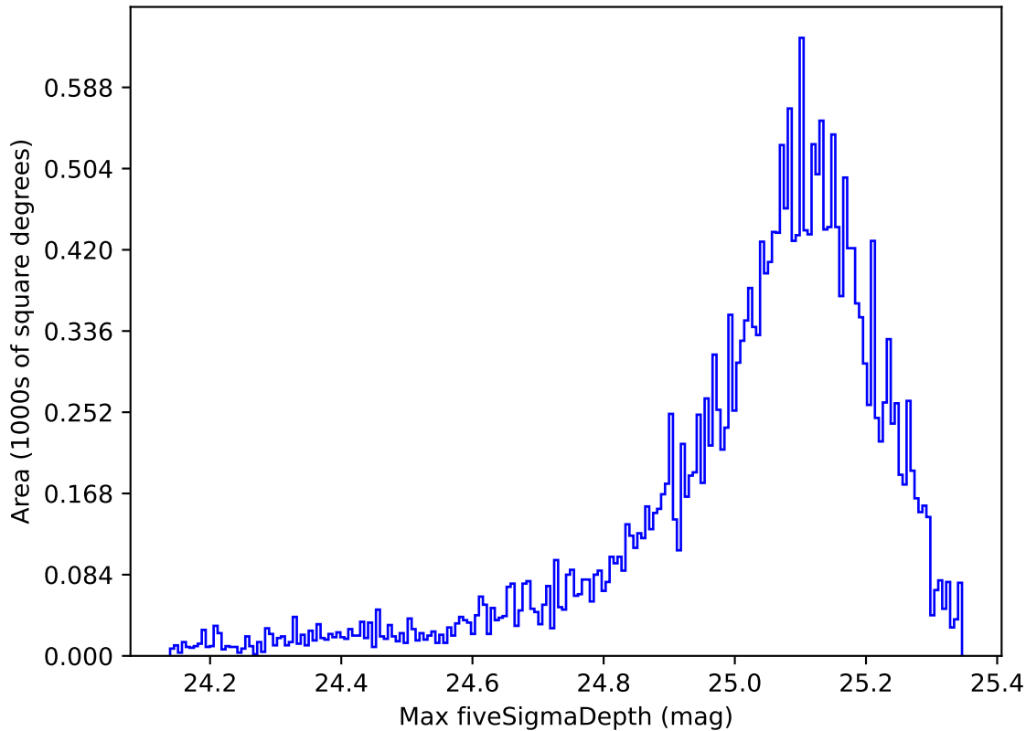
too_ignore_5_1v3.4_10yrs All sky all bands: Max fiveSigmaDepth
