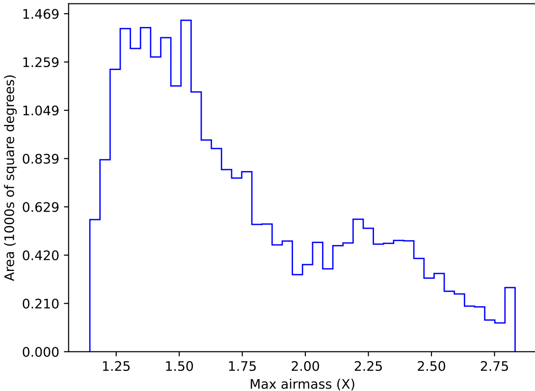
too_ignore_5_1v3.4_10yrs Yr 1 z band: Max airmass
