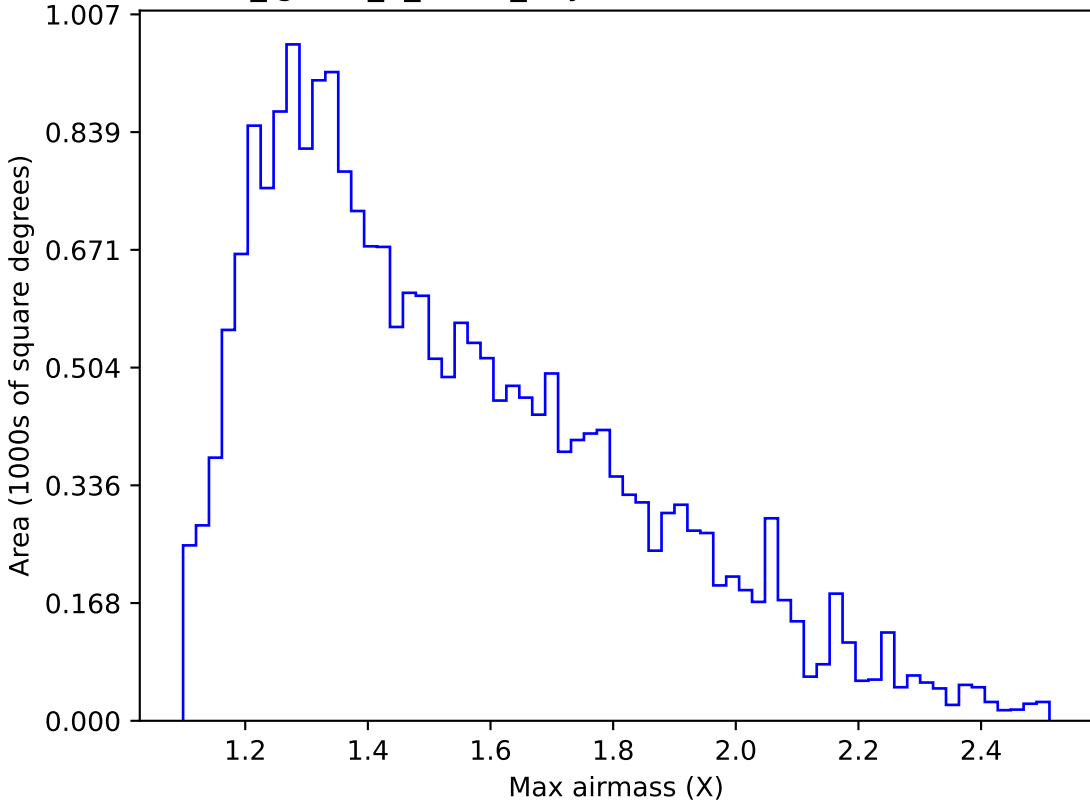
too_ignore_5_1v3.4_10yrs Yr 1 u band: Max airmass
