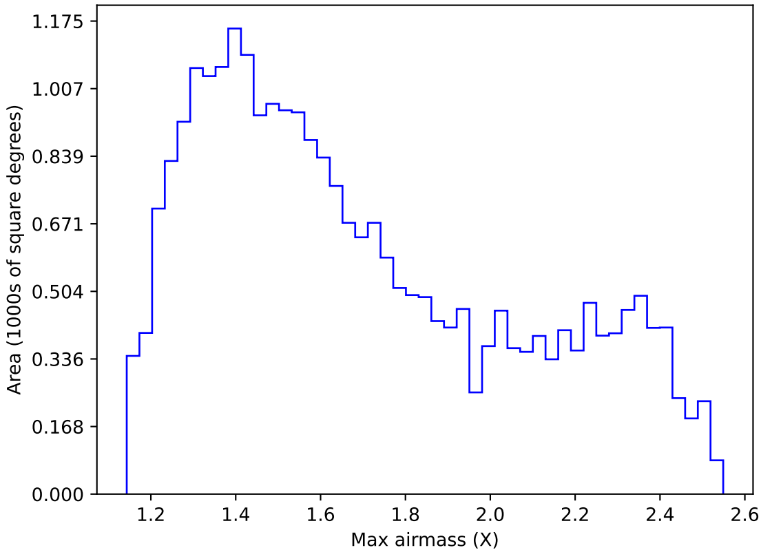
too_ignore_5_1v3.4_10yrs Yr 1 r band: Max airmass
