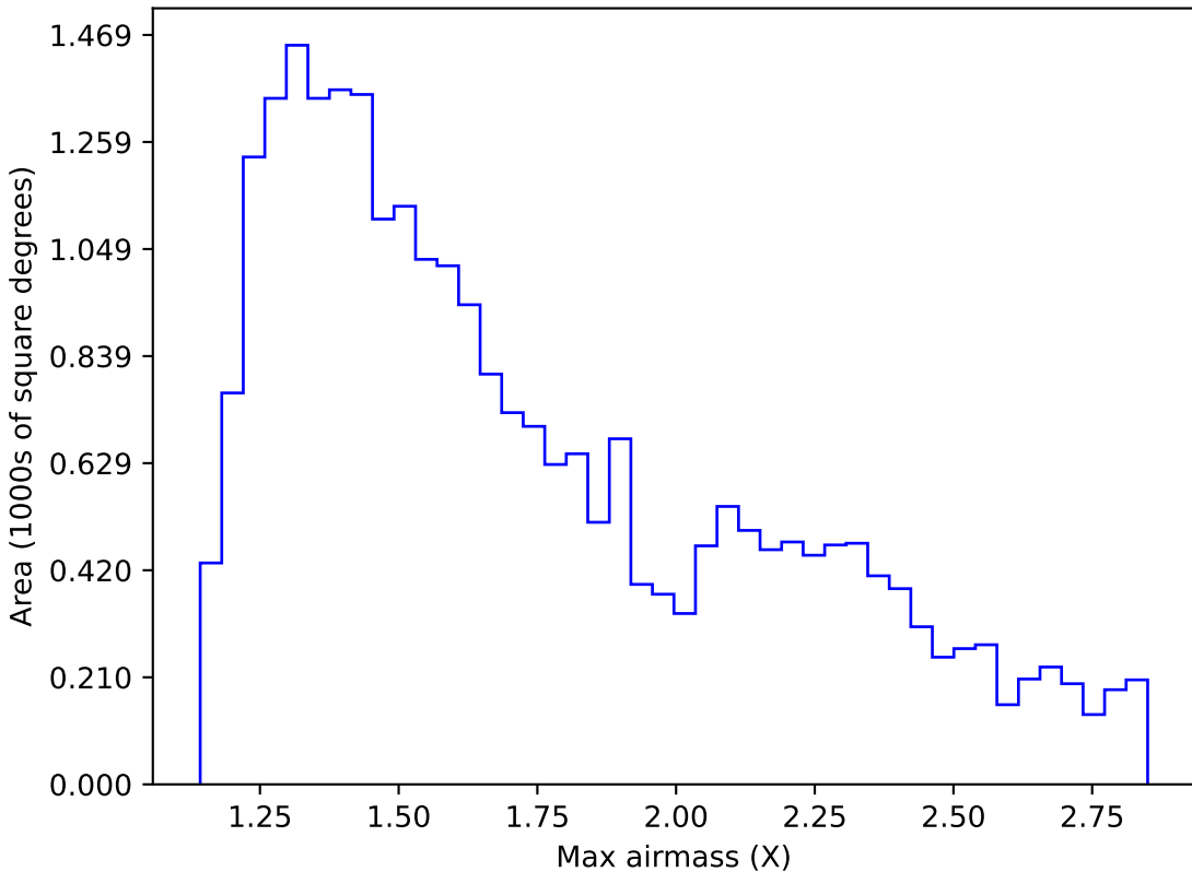
too_ignore_5_1v3.4_10yrs Yr 1 i band: Max airmass
