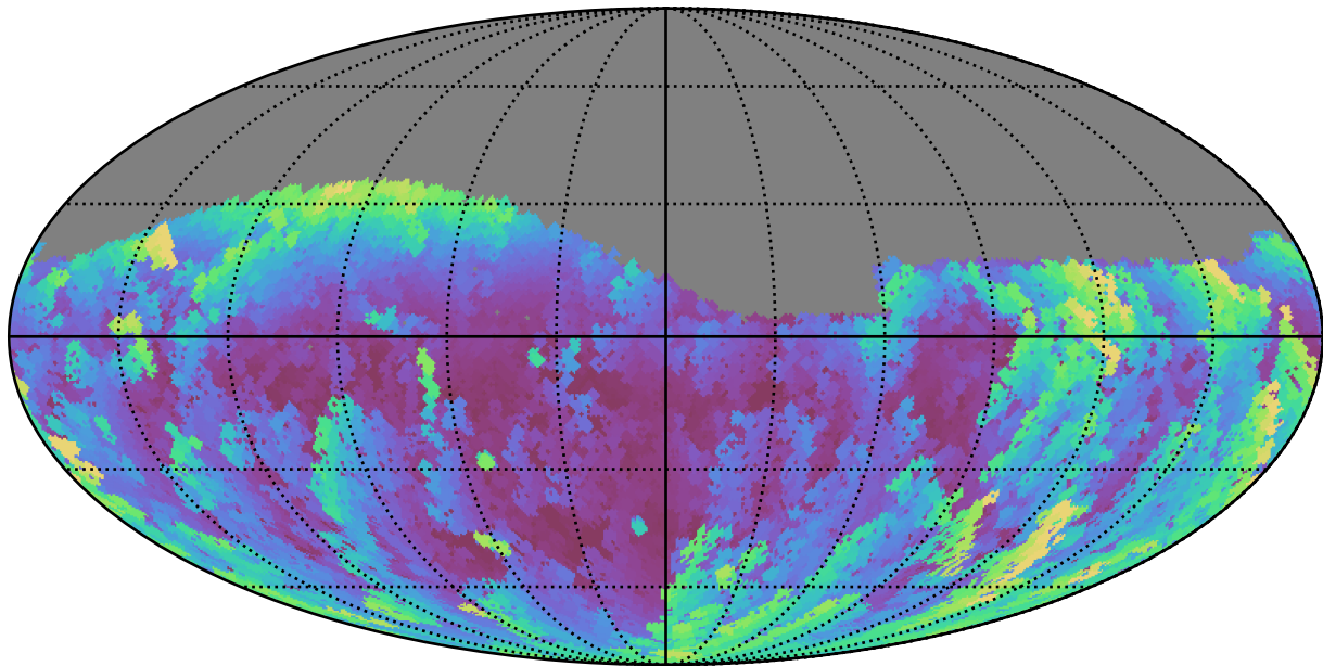
too_ignore_5_1v3.4_10yrs Yr 1 g band: Max airmass
