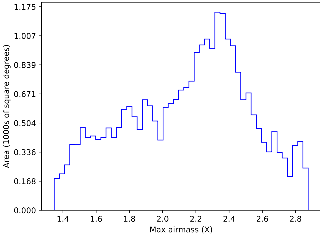
too_ignore_5_1v3.4_10yrs Yr 1 all bands: Max airmass
